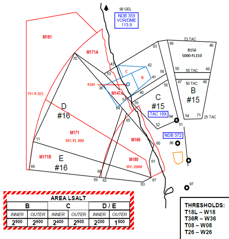
Figure 2. 16 - Nightload Airspace PEARCE_SOP – NIGHT LOAD
