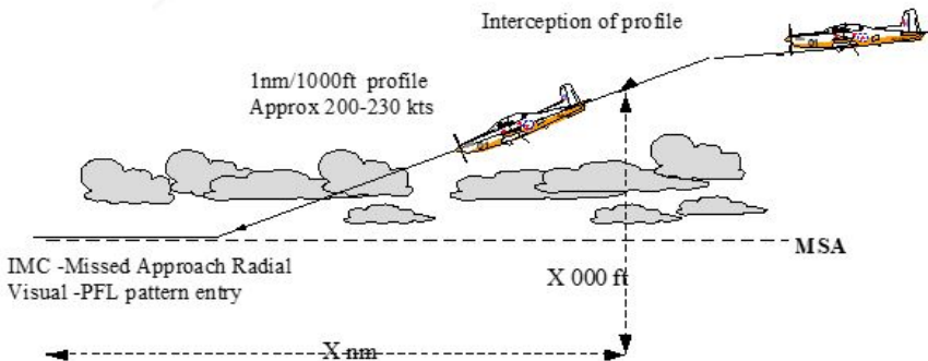
Figure 6 - PFOTAC PROFILE Glide on inbound radial
