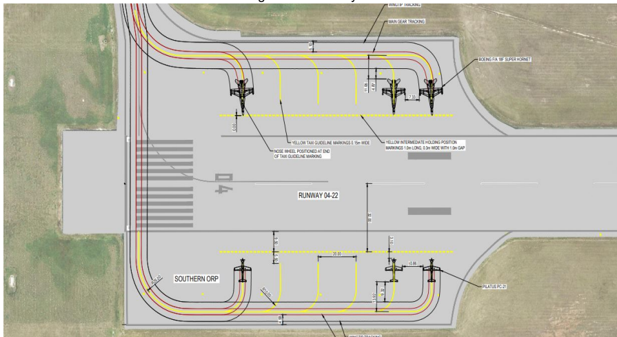
Figure 2 - ORP Layout
