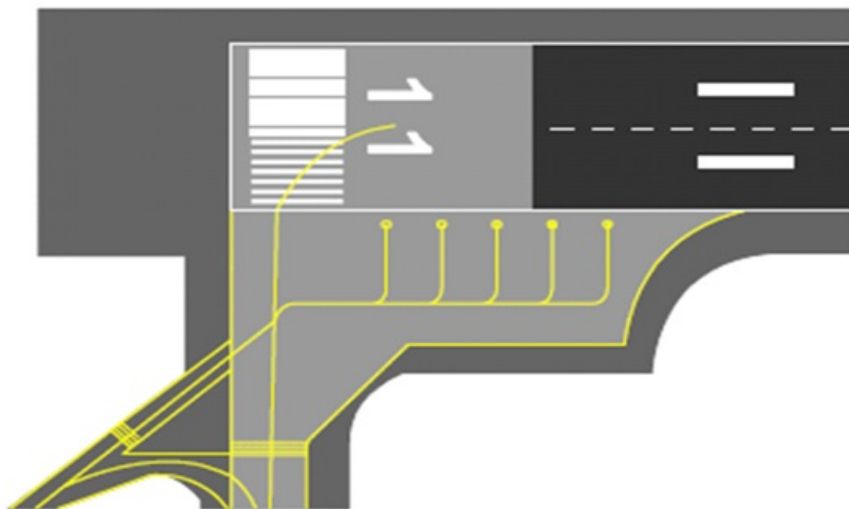
Figure 2 - ORP RWY 11
