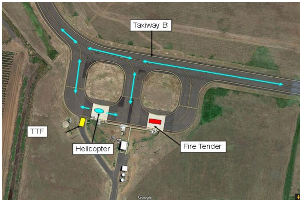
Figure 2: Layout for hot refuelling from bulk tankers
