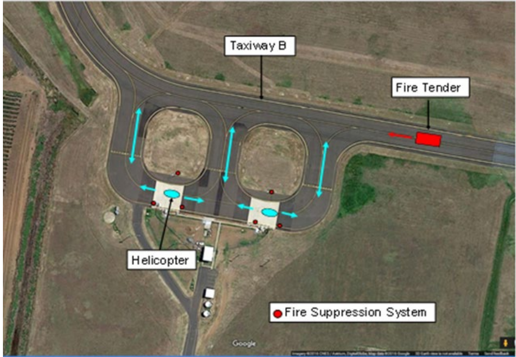
Figure 1: Simultaneous HREF Operations on two refuel pads
