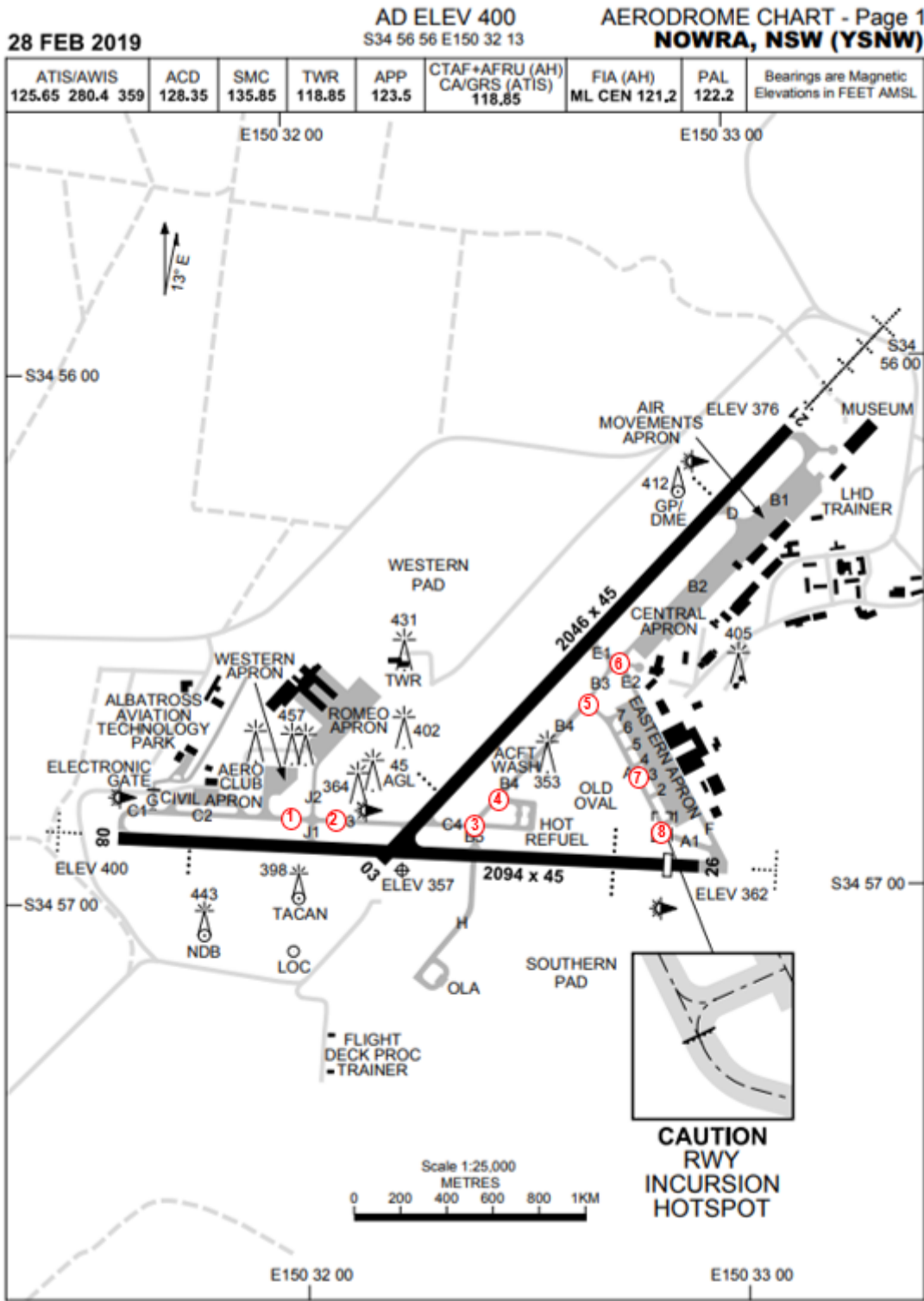
Figure A.1: YSNW aerodrome chart
