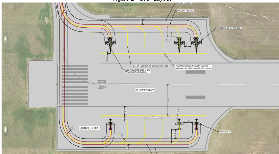
Figure 2 - ORP Layout
