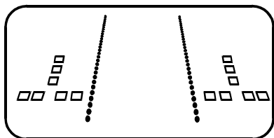
Figure 32 - T-VASIS Signals
