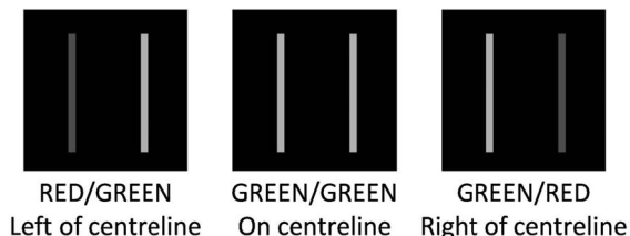
Figure 35 - Centreline Guidance Light Unit
