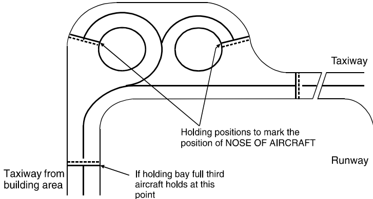
Figure 20 - Holding Bay Markings
