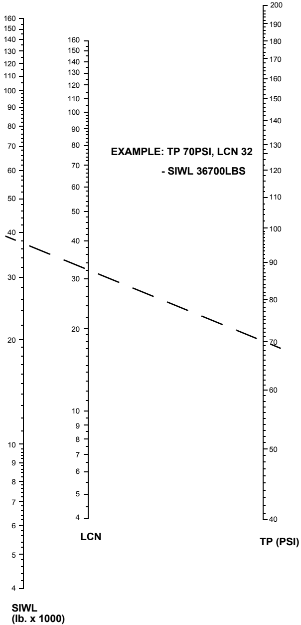
Figure 44 - TP/LCN/SIWL Conversion
