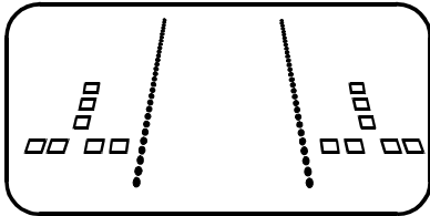
Figure 32 - T-VASIS Signals
