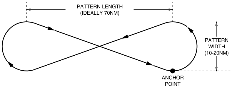
Figure 76.2: AEW&C Figure Eight Orbit Pattern
