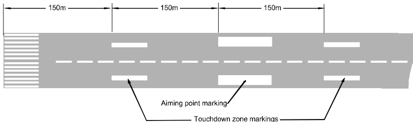
Figure 11 - Aiming Point and Simple Touchdown Zone Markings
