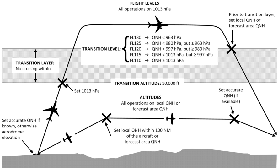
Figure 1 - Altimeter Settings
