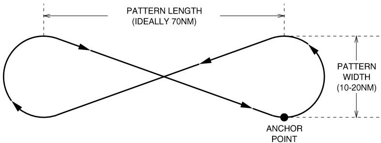
Figure 76.2: AEW&C Figure Eight Orbit Pattern
