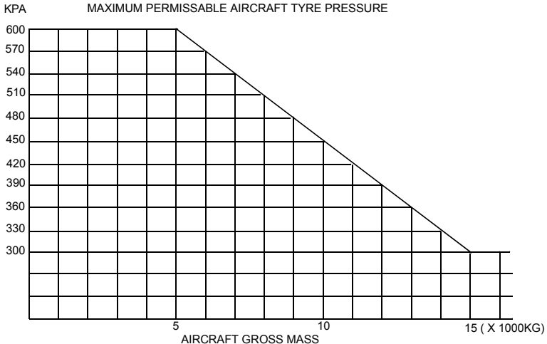
Figure 41 - Aircraft Suitability for Unrated Pavements
