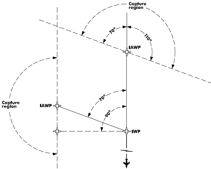
Figure 2.6: RNAV GNSS (or RNP APCH) Capture Regions (Two Initial Approach waypoints)
