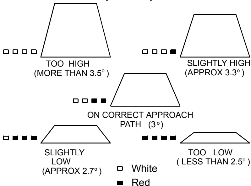
Figure 33 - PAPI signals
