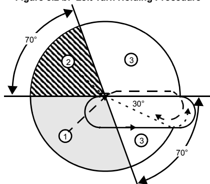
Figure 3.2 b: Left Turn Holding Procedure
