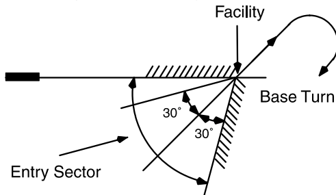
Figure 2.9: Direct Entry to Base Turn
