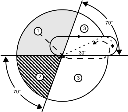
Figure 3.2 a: Right Turn Holding Procedure
