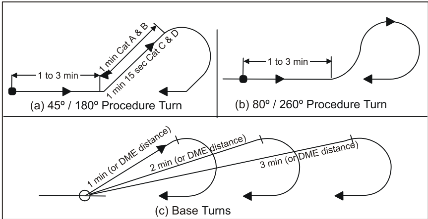
Figure 2.7: Reversal Procedures
