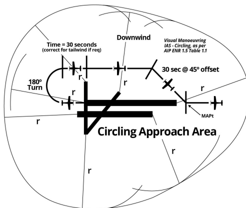
Figure 1.1: Example Visual Circling Obstacle Assessment Area
